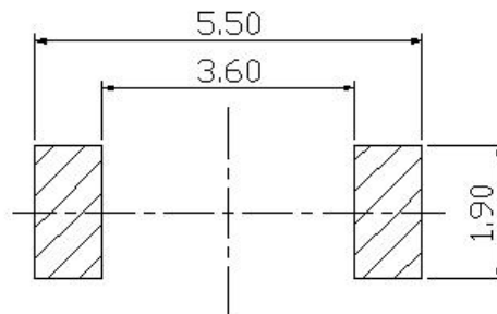
Printed Circuit board dimensions
